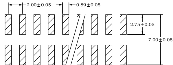
Recommended PCB Layout (Tolerance: ±0.05)
